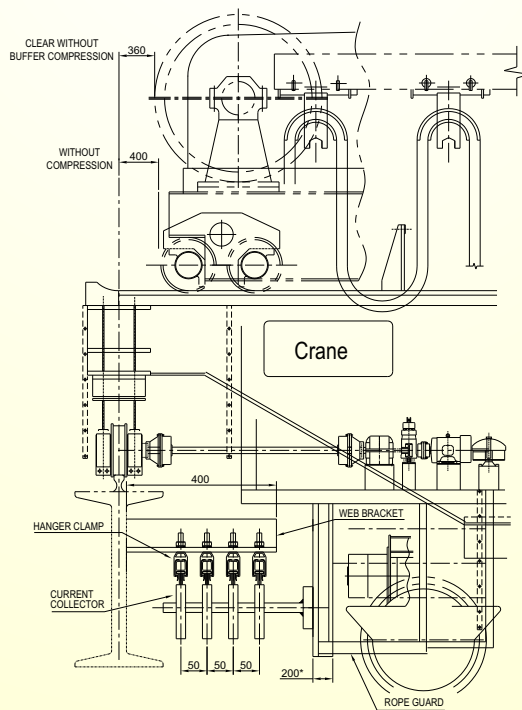
Safeline-C General Arrangement
