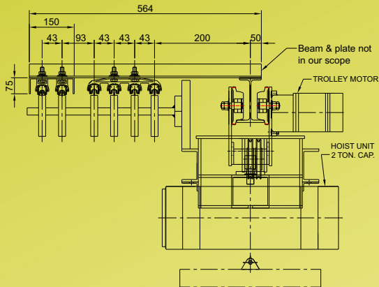
Safeline-W General Arrangement
