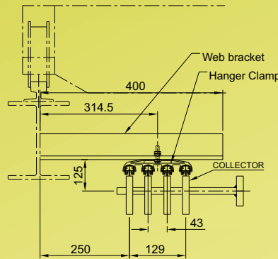
Safeline-W General Arrangement
