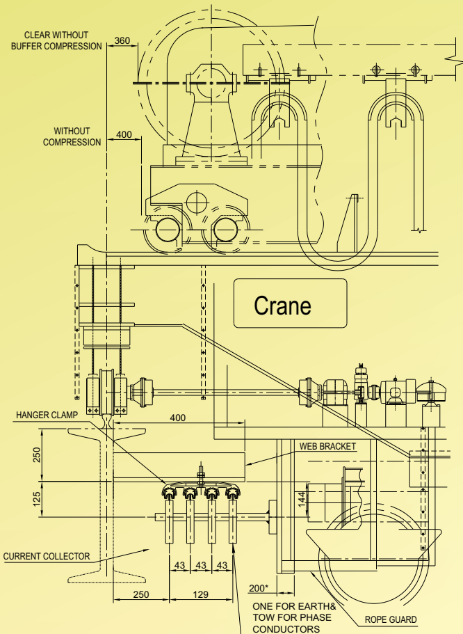
Safeline-W General Arrangement
