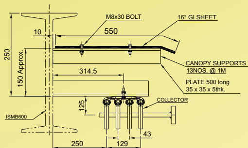
Safeline-W General Arrangement
