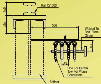
Safeline-W General Arrangement
