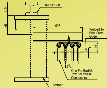
Safeline-W General Arrangement
